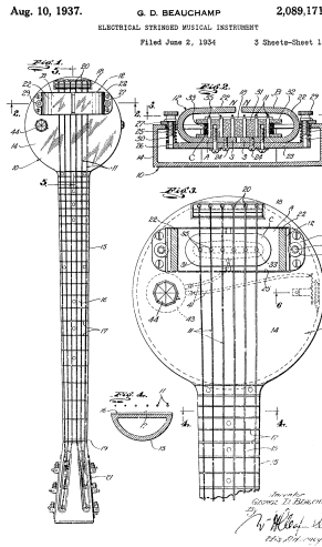
Patent Drawings for the “Frying Pan,” 1937
